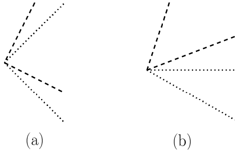
Figure 1: Two possible pairs of special special wedges.
