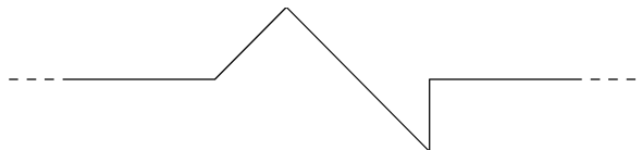
Figure 4: The lower halfplane with a special pair of wedges at its top.
