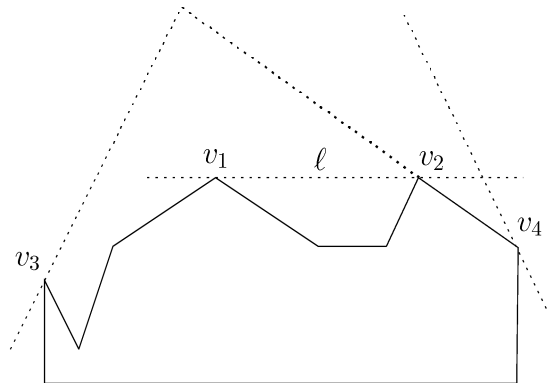
Figure 3: How to find a special pair of wedges.
