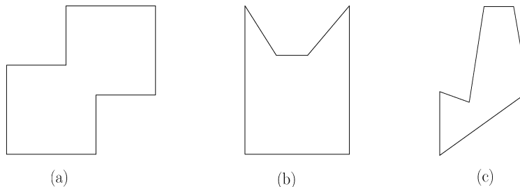
Figure 6: Three different polygons. (a): totally-cover-decomposable (hence, also plane-cover-decomposable), (b): not plane-cover-decomposable, (hence neither totally-cover-decomposable), (c): not totally-cover-decomposable, but not known if plane-cover-decomposable.
