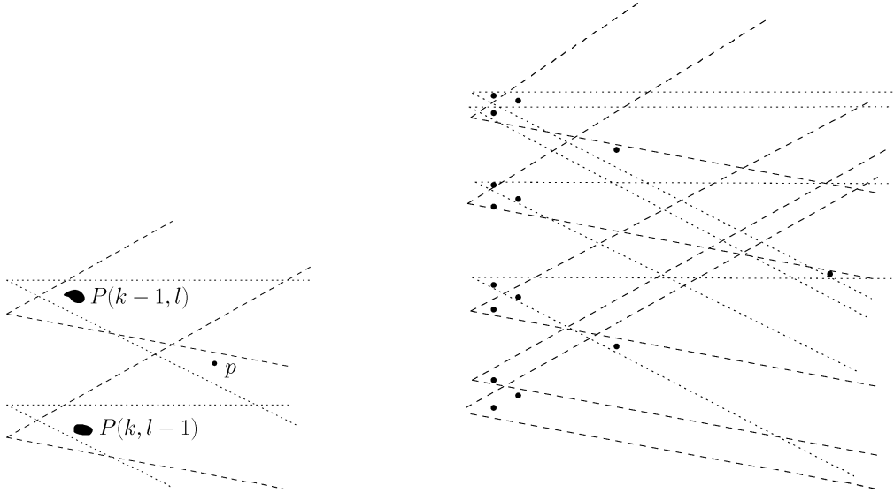
Figure 2: Sketch of one step of the induction and the first few steps.
